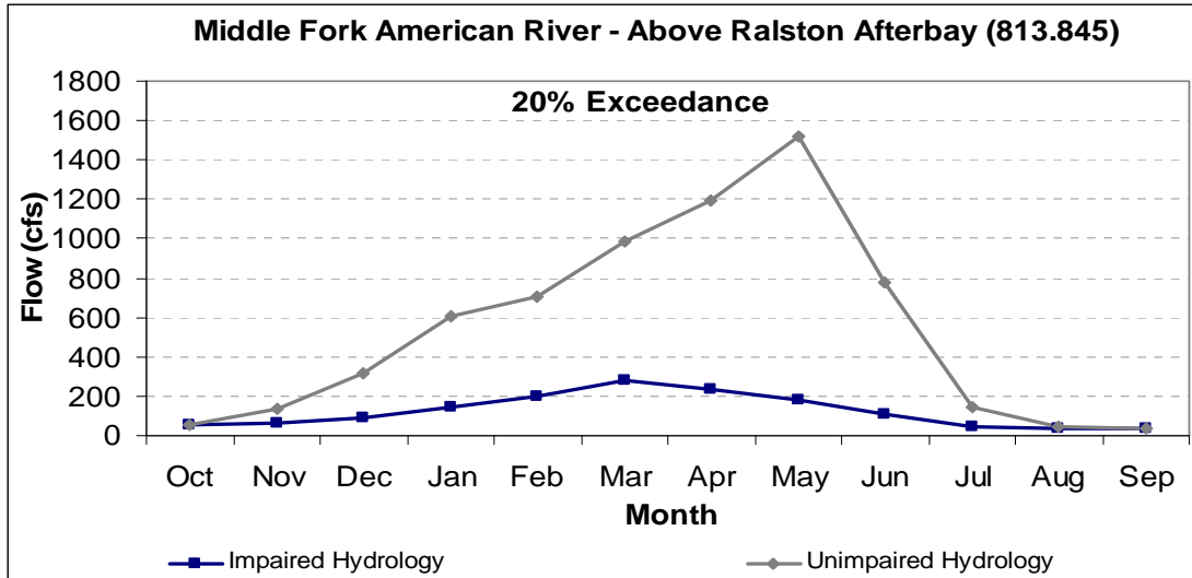
Figure 7.3-4. Graphs of Monthly Exceedance Curves (20%, 50%, and 80%) for Selected Locations in Waters Associated with the Middle Fork American River Project (continued).
