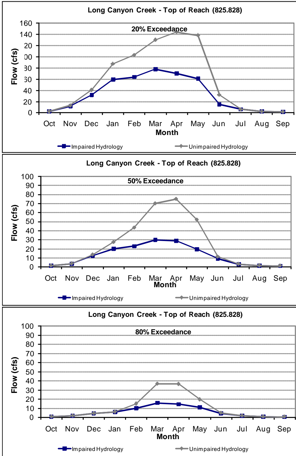
Figure 7.3-4. Graphs of Monthly Exceedance Curves (20%, 50%, and 80%) for Selected Locations in Waters Associated with the Middle Fork American River Project (continued).
