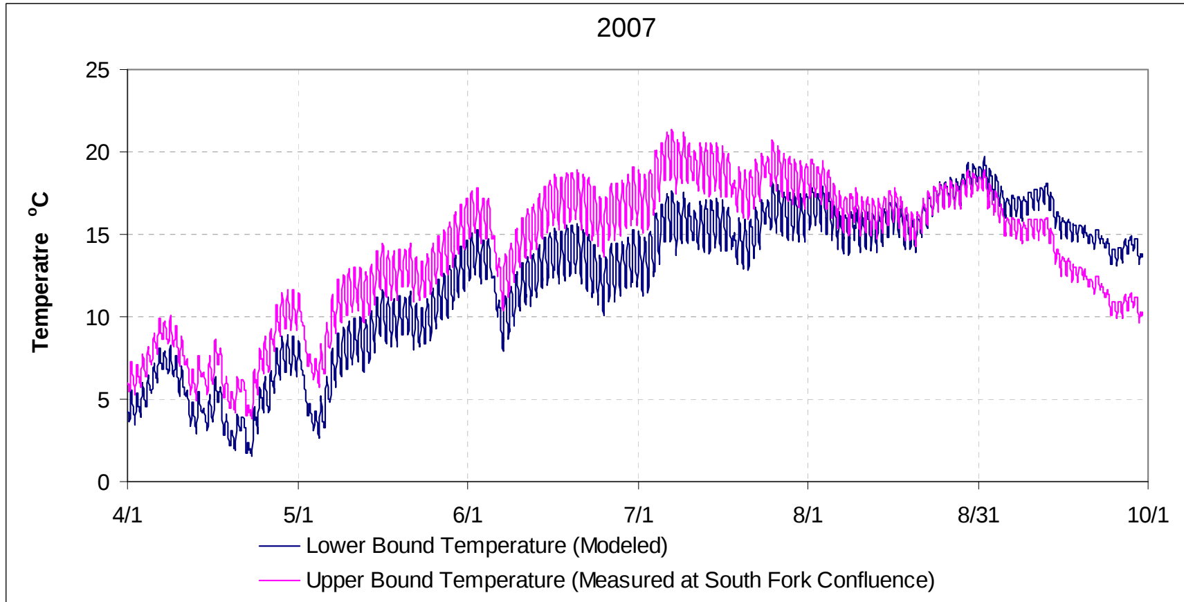
Figure 1. Estimated Upper and Lower Bounding Temperatures for South Fork Rubicon Inflow to the Rubicon River 2007.
