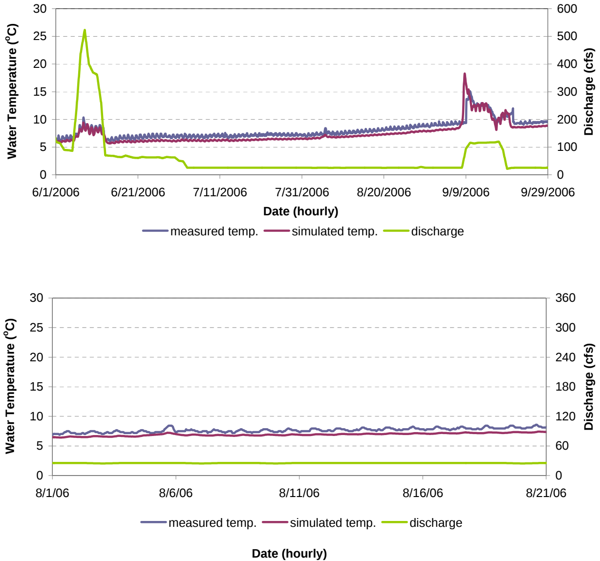
Figure F-9. Water Temperature Model Calibration Results for MF 35.5 in the Middle Fork Interbay to Ralston Afterbay Reach of the Middle Fork American River for June 1 - September 30, 2006 (Top) and August 1 - August 21, 2006 (Bottom).
