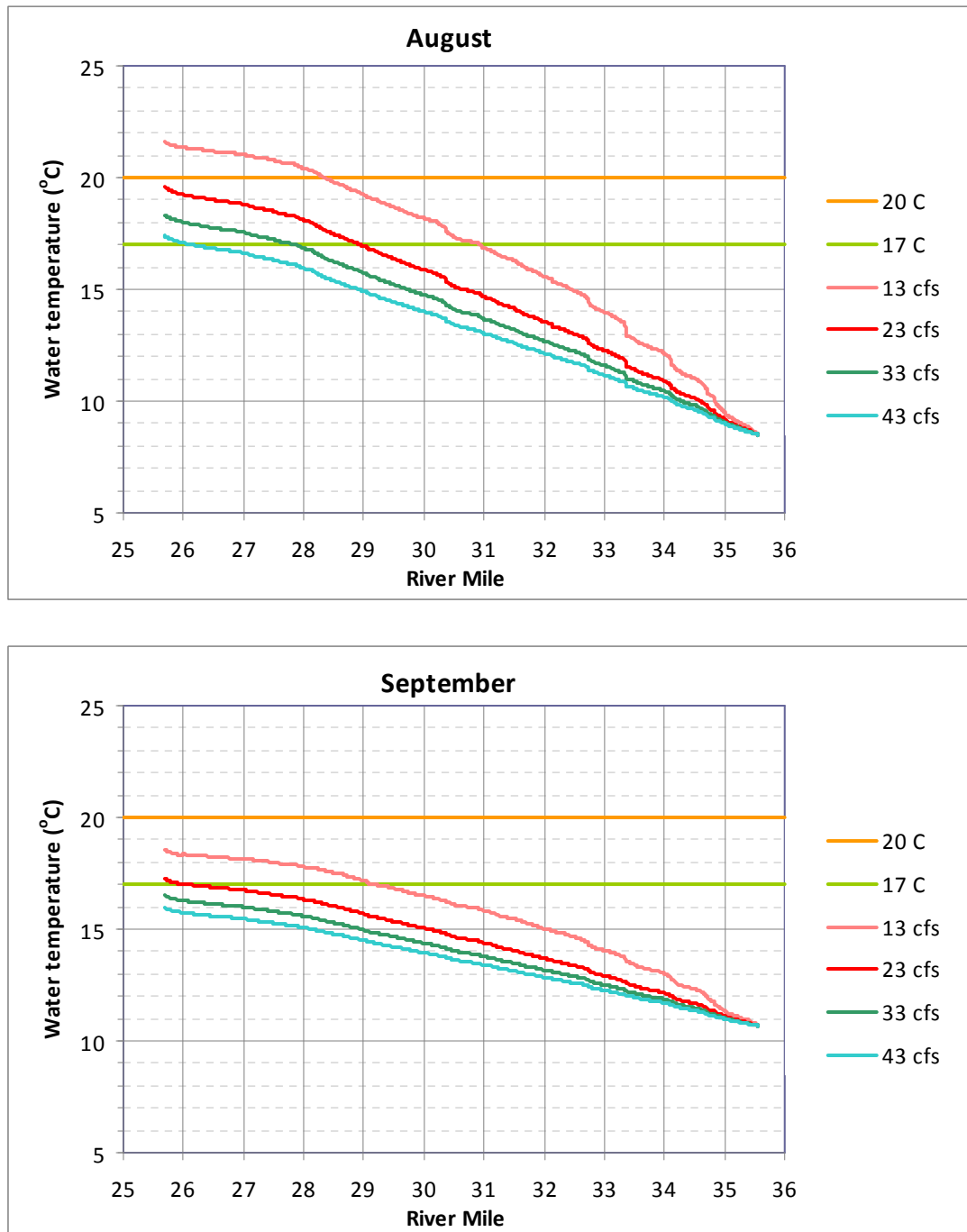
Figure 3b. Middle Fork American River below Middle Fork Interbay Modeled Sensitivity Longitudinal Profiles—August (top) and September (bottom).
