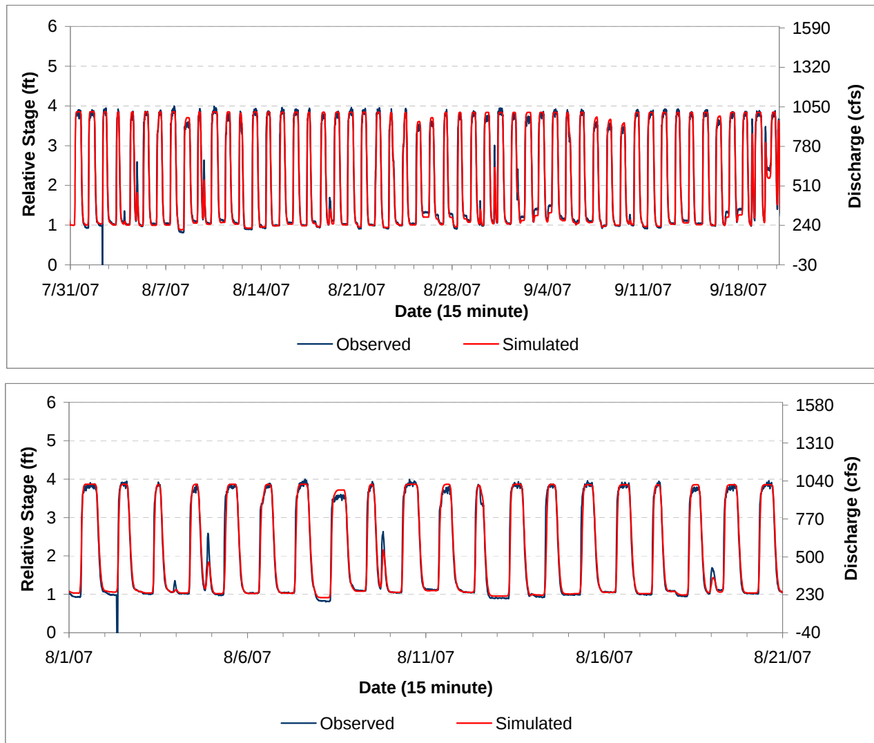
Figure AQ 4-17. RMA-2 Hydrodynamics Calibration Results for the Peaking Reach -- Cache Rock RM 19.3.
