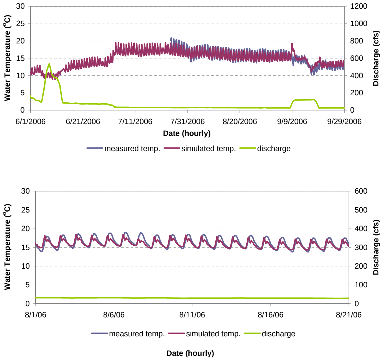
Figure F-11. Water Temperature Model Calibration Results for MF 29.4 in the Middle Fork Interbay to Ralston Afterbay Reach of the Middle Fork American River for June 1 - September 30, 2006 (Top) and August 1 - August 21, 2006 (Bottom).
