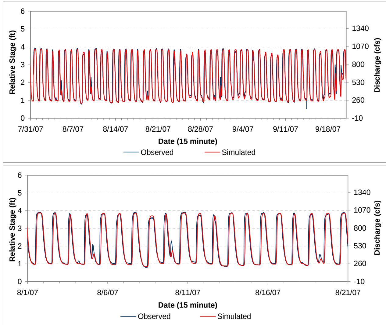
Figure AQ 4-19. RMA-2 Hydrodynamics Calibration Results for the Peaking Reach -- Drivers Flat RM 9.5.
