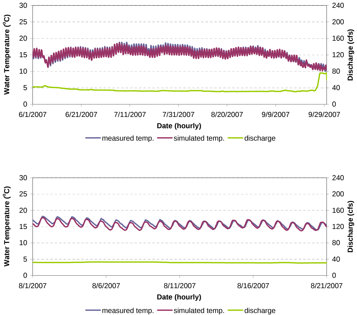
Figure F-22. Water Temperature Model Calibration Results for RR 22.5 in the Hell Hole Reservoir to Ralston Afterbay Reach of the Rubicon River for June 1 - September 30, 2007 (Top) and August 1 - August 21, 2007 (Bottom).
