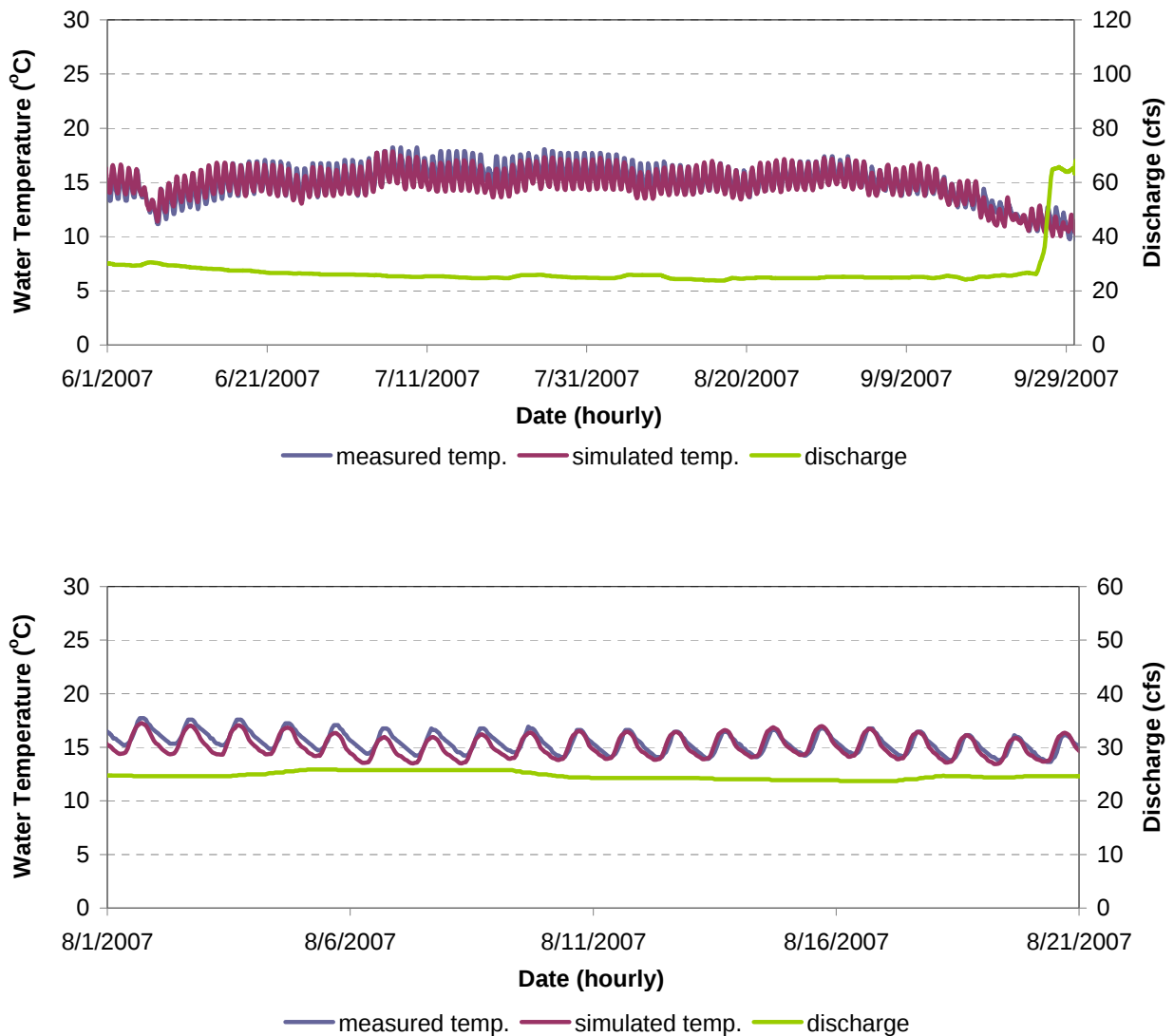
Figure F-20. Water Temperature Model Calibration Results for RR 22.7 in the Hell Hole Reservoir to Ralston Afetrbay Reach of the Rubicon River for June 1 - September 30, 2007 (Top) and August 1 - August 21, 2007 (Bottom).
