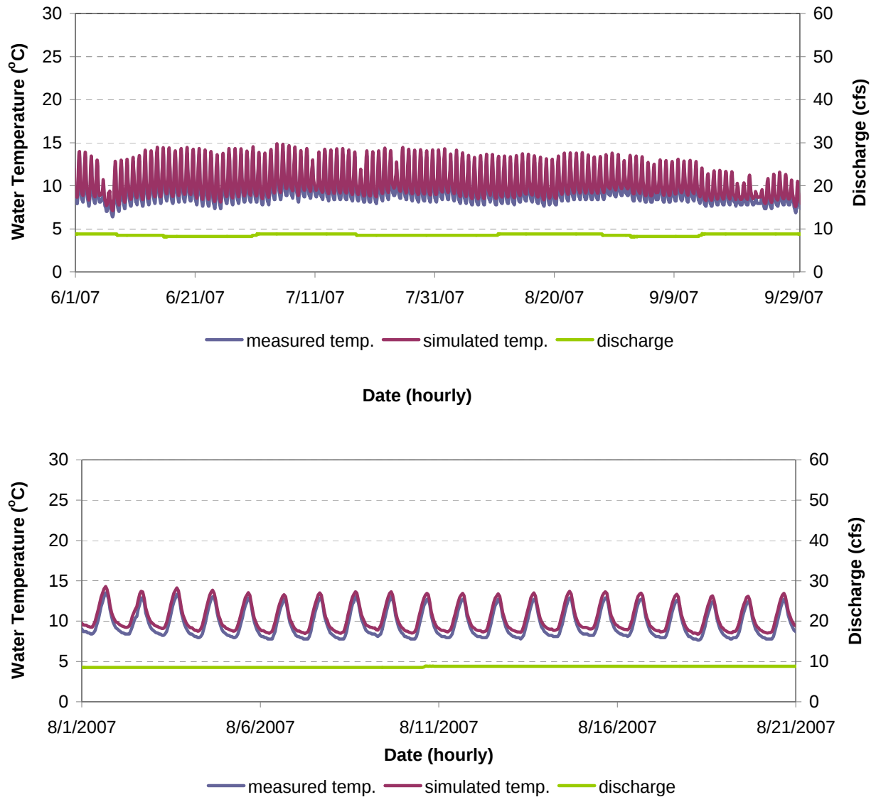
Figure F-2. Water Temperature Model Calibration Results for MF 46.6 in the French Meadows Reservoir to Middle Fork Interbay Reach of the Middle Fork American River for June 1 - September 30, 2007 (Top) and August 1 - August 21, 2007 (Bottom).
