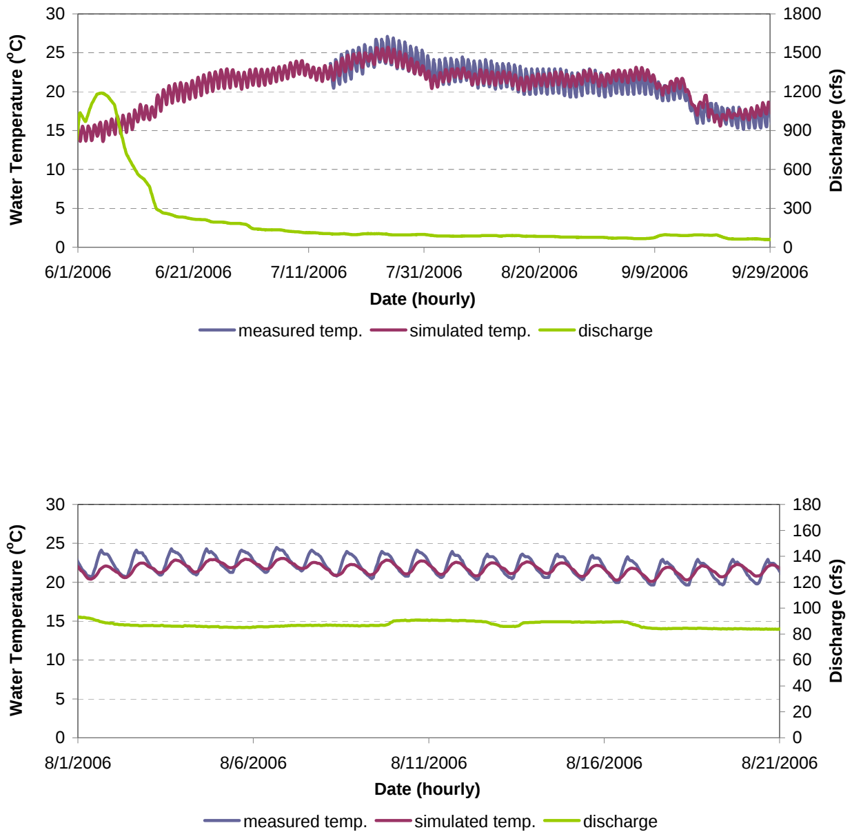
Figure F-29. Water Temperature Model Calibration Results for RR 0.7 in the Hell Hole Reservoir to Ralston Afterbay Reach of the Rubicon River for June 1 - September 30, 2006 (Top) and August 1 - August 21, 2006 (Bottom).
