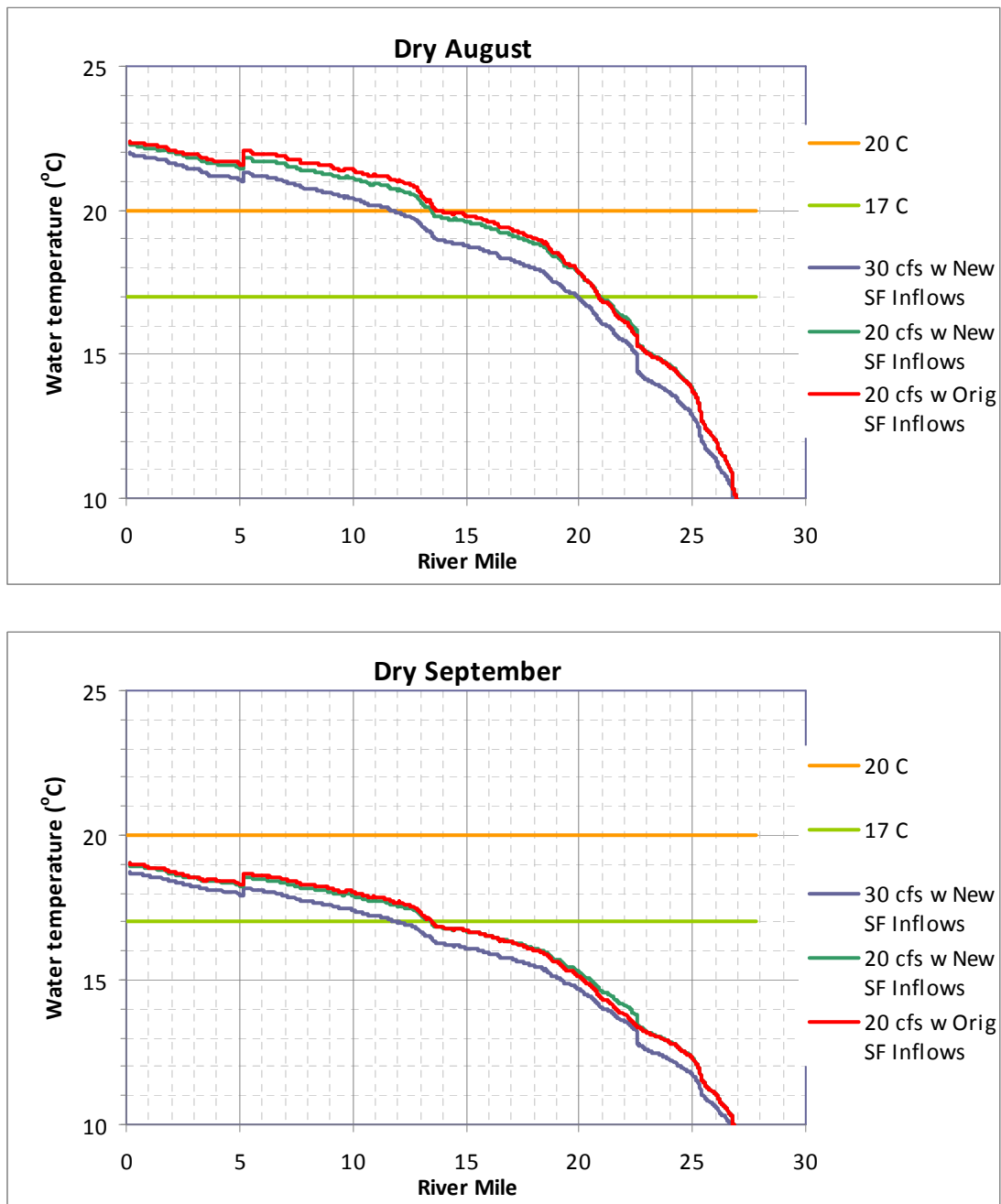
Figure 5b. Rubicon River Dry Water Year Modeled Sensitivity Longitudinal Profiles—August (top) and September (bottom).
