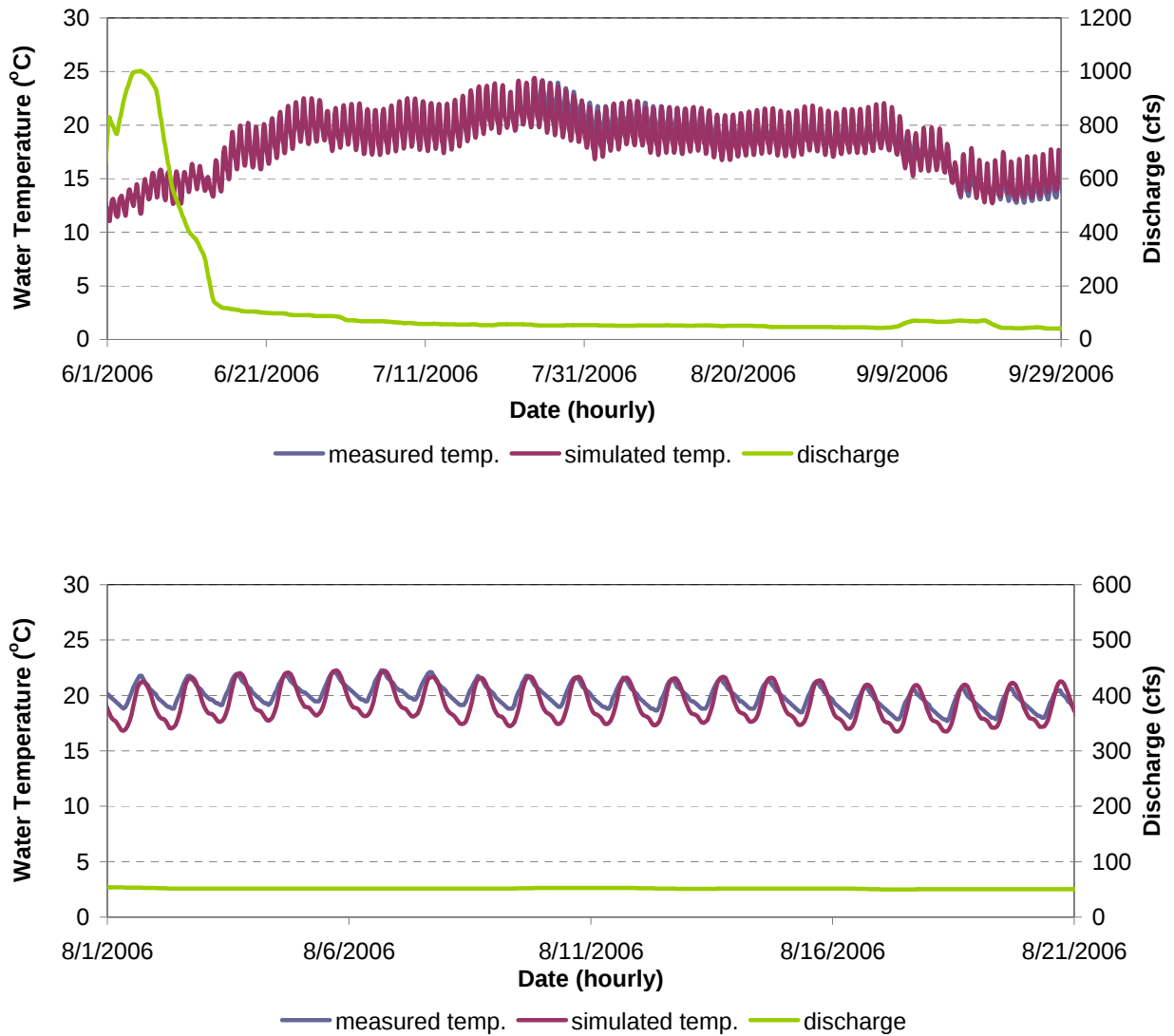
Figure F-23. Water Temperature Model Calibration Results for RR 14.3 in the Hell Hole Reservoir to Ralston Afterbay Reach of the Rubicon River for the June 1 - September 30, 2006 (Top) and August 1 - August 21, 2006 (Bottom).
