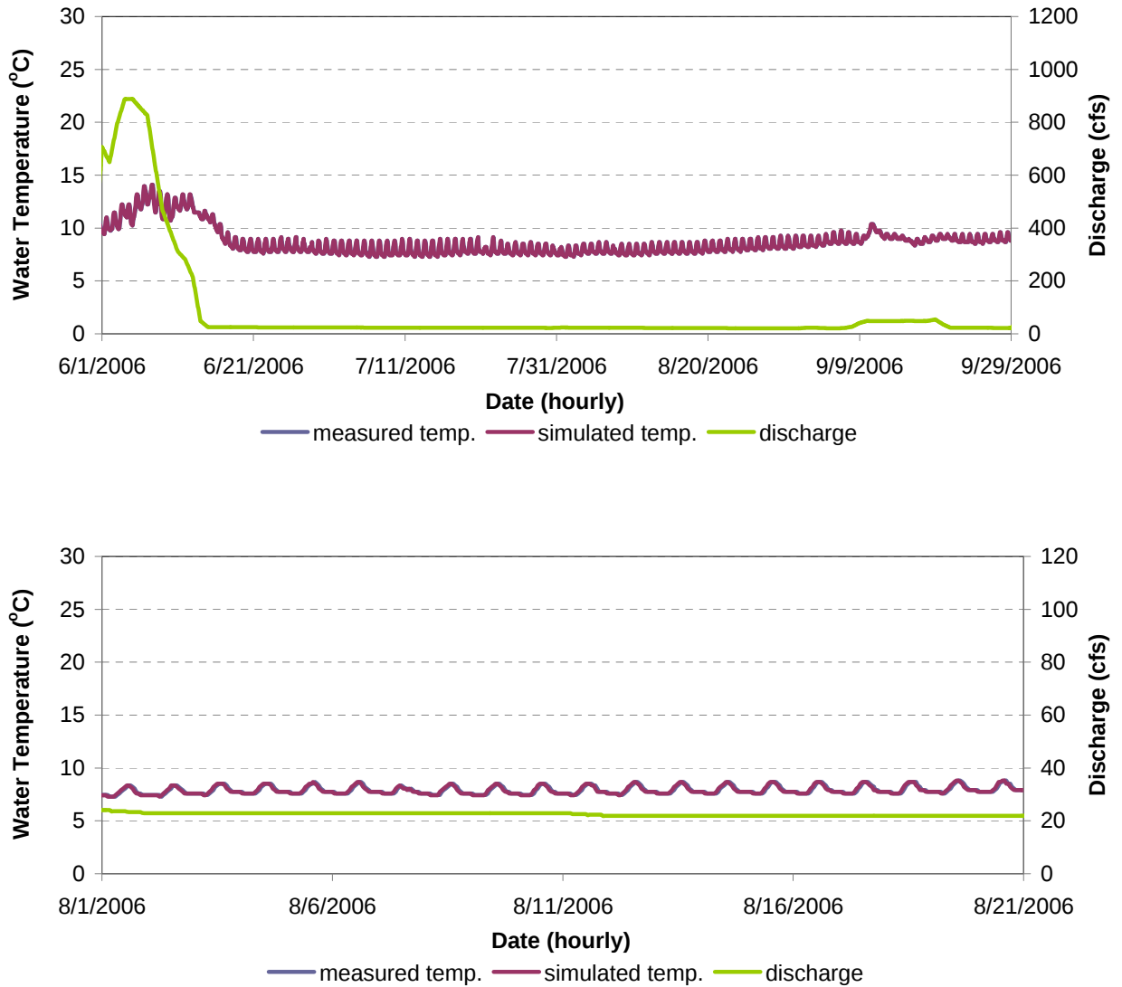
Figure F-15. Water Temperature Model Calibration Results for RR 28.8 in the Hell Hole Reservoir to Ralston Afterbay Reach of the Rubicon River for June 1 - September 30, 2006 (Top) and August 1 - August 21, 2006 (Bottom).
