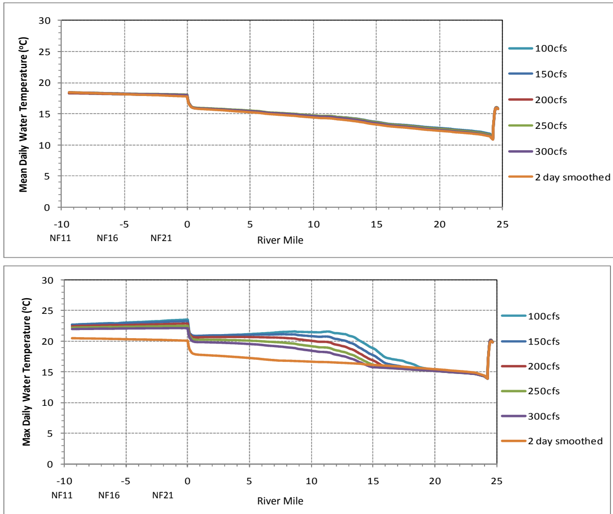
Figure H-30. Middle Fork American River Peaking Reach Longitudinal Profiles of Daily Mean (Top) and Maximum (Bottom) Water Temperature for the First Week of July, 2007 for Various Discharge Scenarios (100 cfs, 150 cfs, 200 cfs, 250 cfs and 300 cfs Minimum Discharge and 2-Day Average Discharge).
