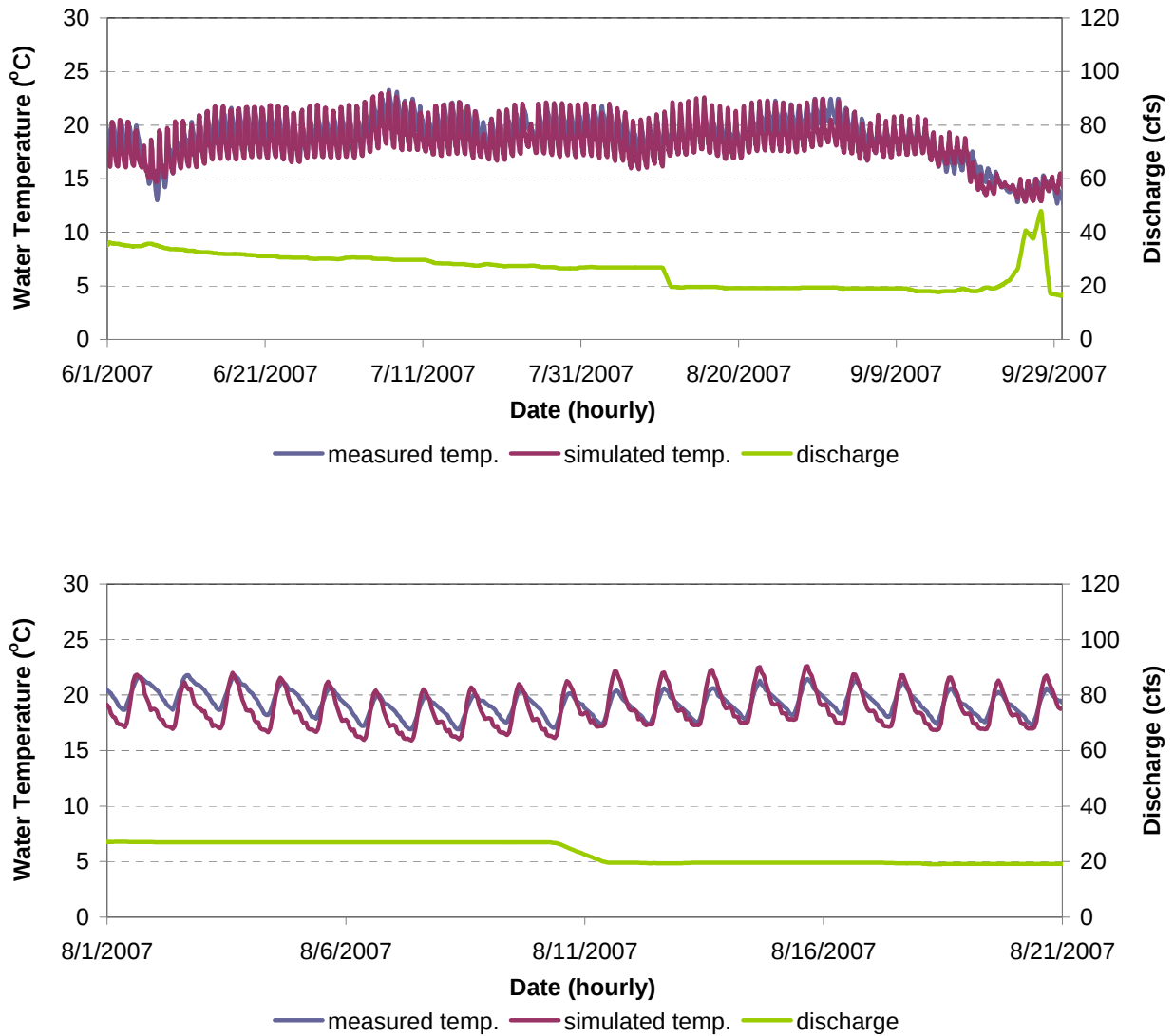
Figure F-14. Water Temperature Model Calibration Results for MF 26.0 in the Middle Fork Interbay to Ralston Afterbay Reach of the Middle Fork American River for June 1 - September 30, 2007 (Top) and August 1 - August 21, 2007 (Bottom).
