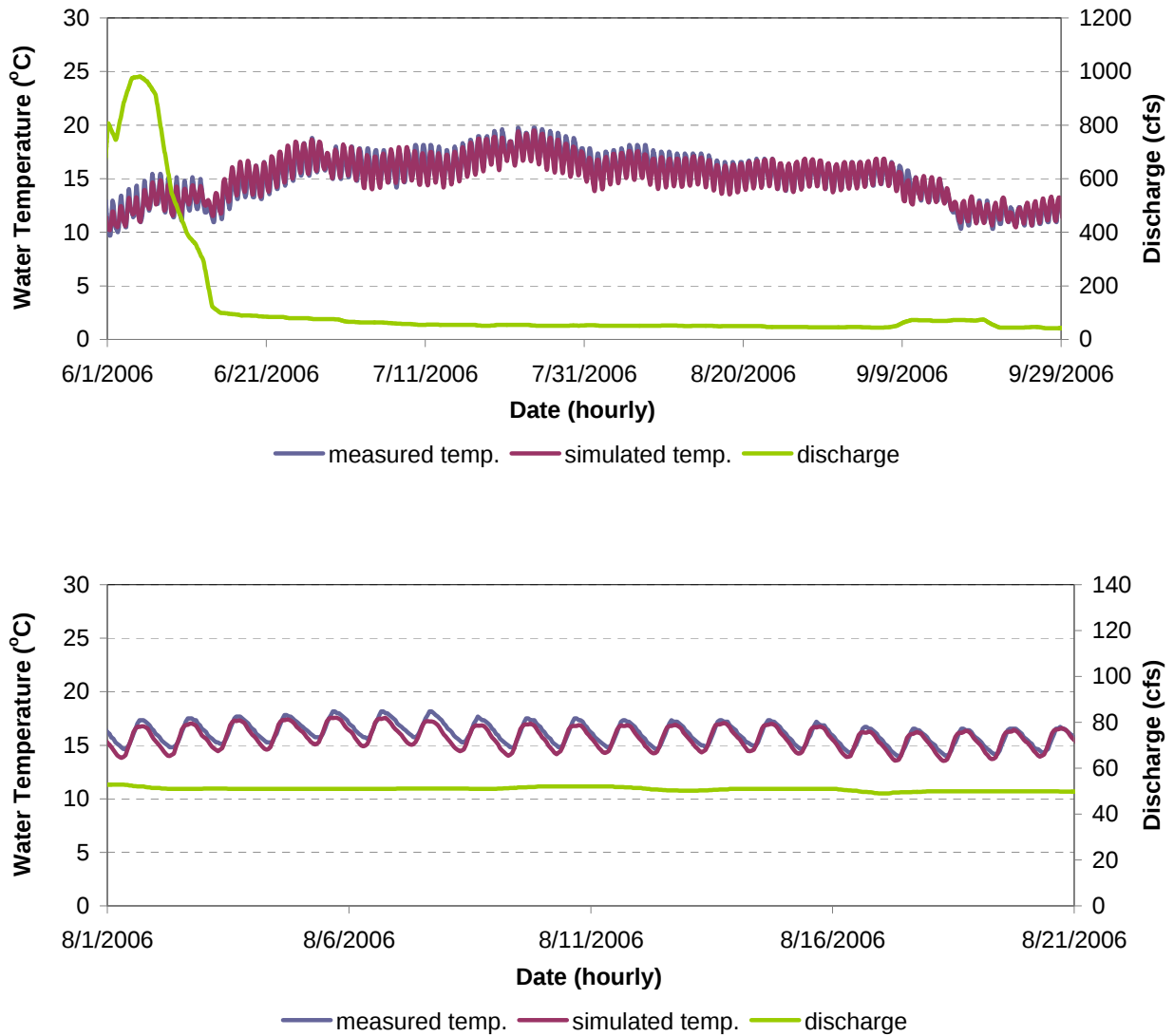
Figure F-21. Water Temperature Model Calibration Results for RR 22.5 in the Hell Hole Reservoir to Ralston Afterbay Reach of the Rubicon River for June 1 - September 30, 2006 (Top) and August 1 - August 21, 2006 (Bottom).
