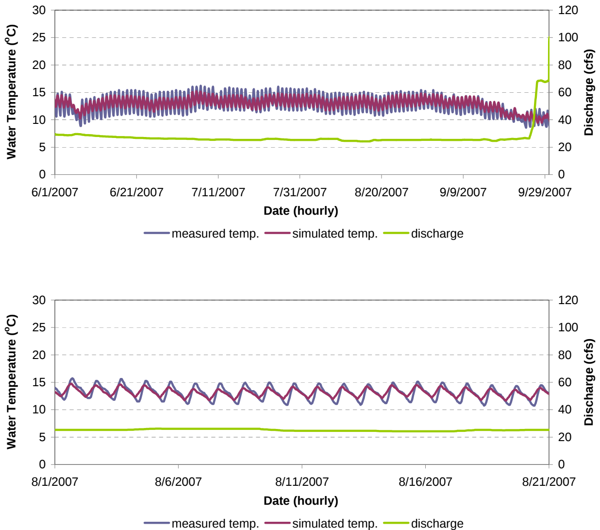
Figure F-18. Water Temperature Model Calibration Results for RR 25.3 in the Hell Hole Reservoir to Ralston Afterbay Reach of the Rubicon River for June 1 - September 30, 2007 (Top) and August 1 - August 21, 2007 (Bottom).
