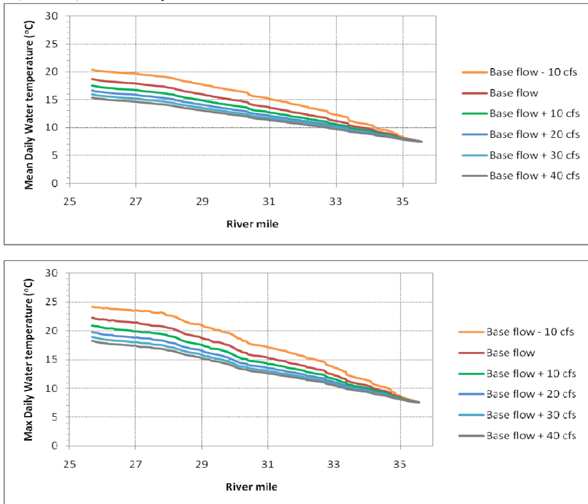
Figure H-12. Middle Fork American River from Middle Fork Interbay to Ralston Afterbay Longitudinal Profiles of Daily Mean (Top) and Maximum (Bottom) Water Temperature for the First Week of August, 2007 for Various Discharge Scenarios (-10 cfs, 0 cfs, +10 cfs, +20 cfs, +30 cfs, and +40 cfs).
