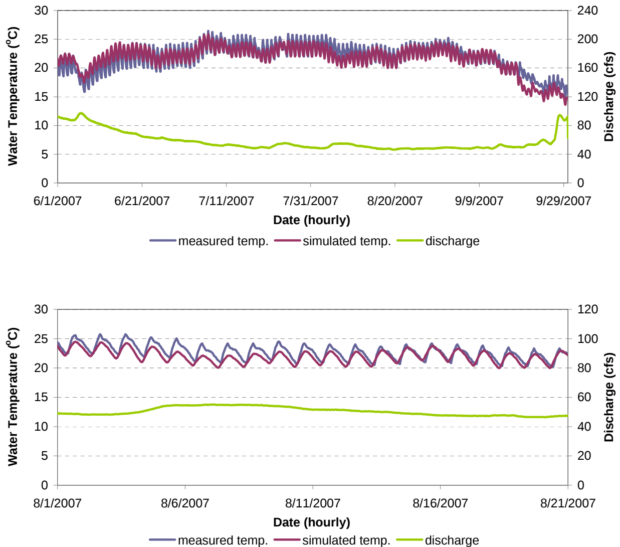
Figure F-30. Water Temperature Model Calibration Results for RR 0.7 in the Hell Hole Reservoir to Ralston Afterbay Reach of the Rubicon River for June 1 - September 30, 2007 (Top) and August 1 - August 21, 2007 (Bottom).
