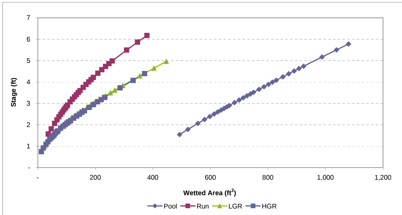
Figure B-3a. Stage-Wetted Area Relationships for Habitat Types in the Ralston Afterbay to Folsom Reservoir Reach of the Middle Fork and the North Fork of the American River.
