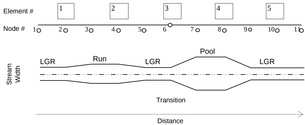
Figure AQ 4-6. Example Computational Mesh for a Representative River Reach, Showing Habitat Types on an Element-by-Element Basis. Node Spacing is 25 m.
