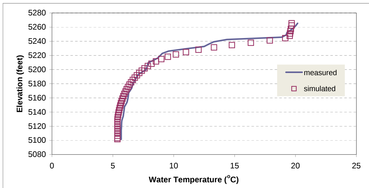
Figure E-5. Calibration Data for French Meadows Reservoir on July 6, 2006 for Segment 17 (Temperature Model) and Vertical Profile Sampling Location FM2.
