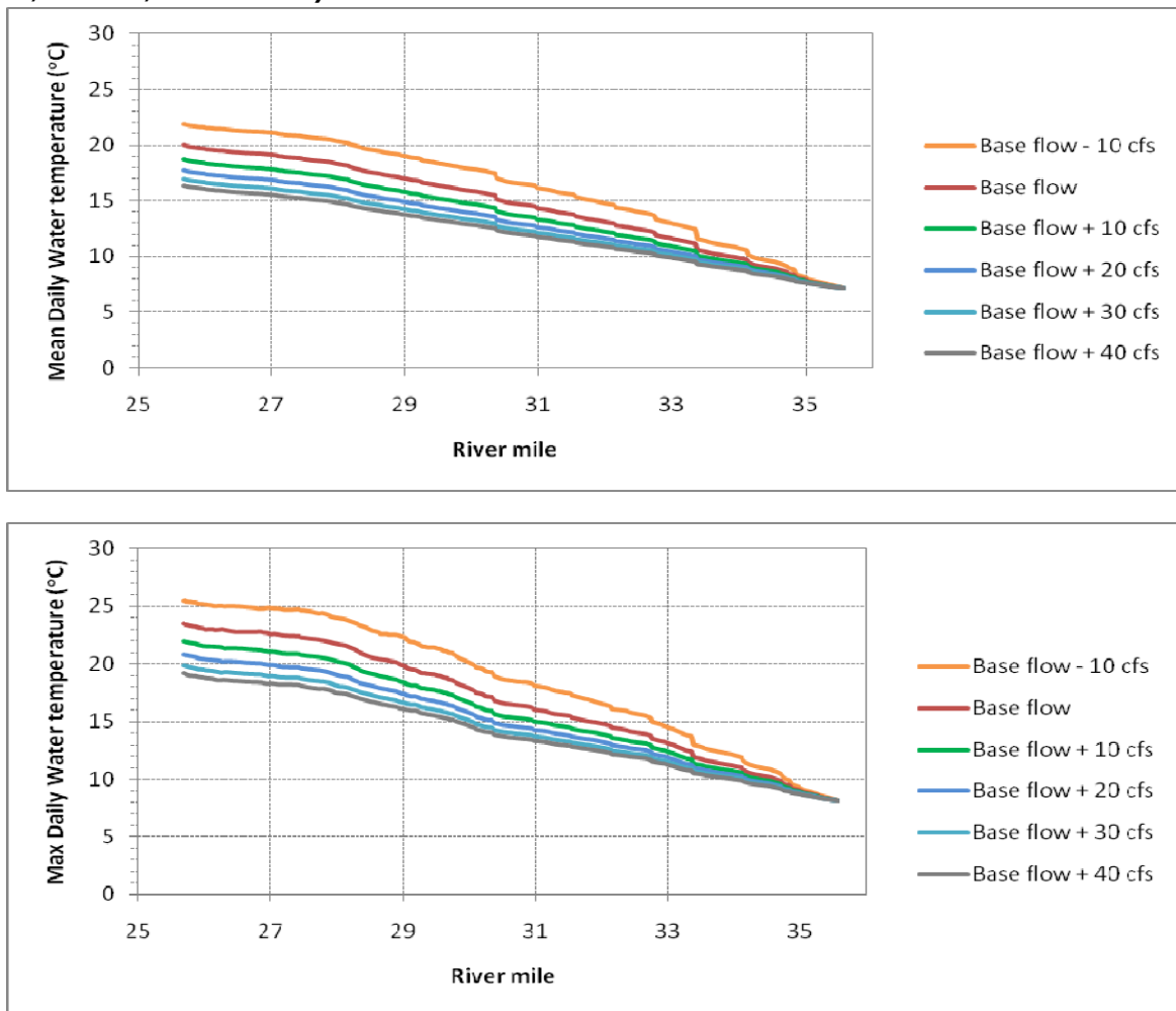
Figure H-11. Middle Fork American River from Middle Fork Interbay to Ralston Afterbay Longitudinal Profiles of Daily Mean (Top) and Maximum (Bottom) Water Temperature for the First Week of July, 2007 for Various Discharge Scenarios (-10 cfs, 0 cfs, +10 cfs, +20 cfs, +30 cfs, and +40 cfs).
