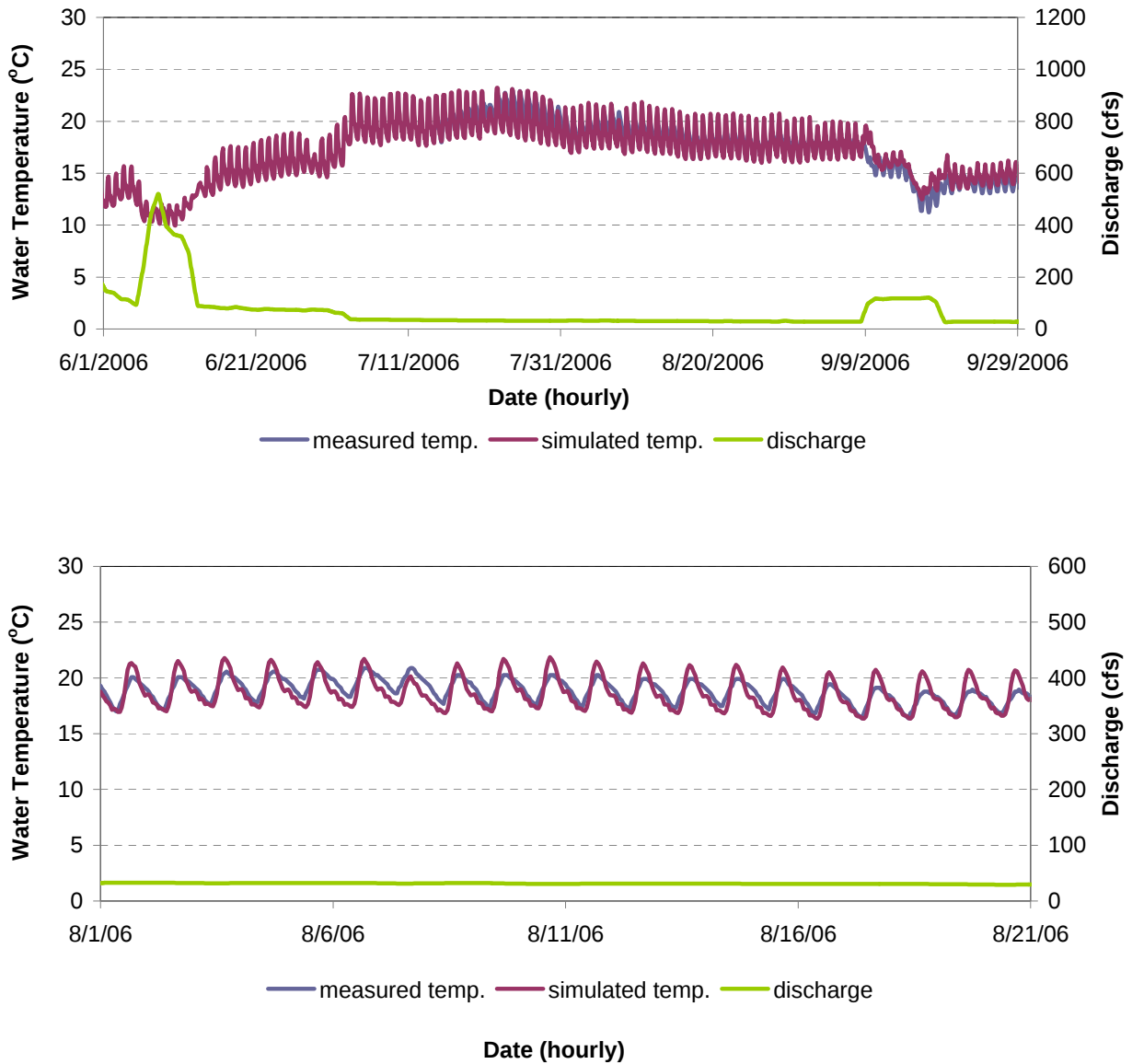
Figure F-13. Water Temperature Model Calibration Results for MF 26.0 in the Middle Fork Interbay to Ralston Afterbay Reach of the Middle Fork American River for June 1 - September 30, 2006 (Top) and August 1 - August 21, 2006 (Bottom).
