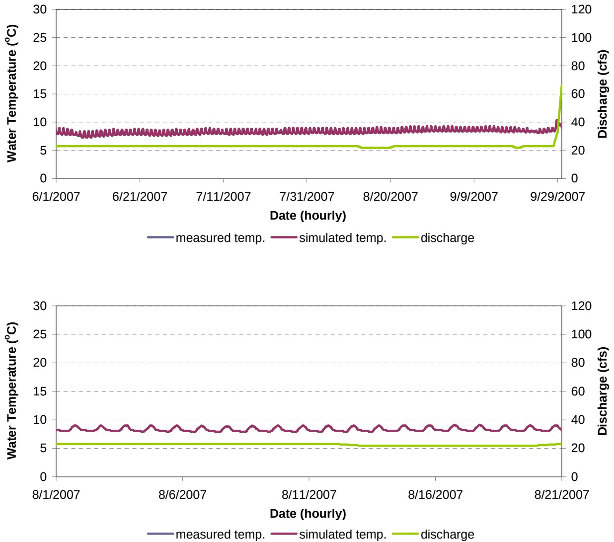
Figure F-16. Water Temperature Model Calibration Results for RR 28.8 in the Hell Hole Reservoir to Ralston Afterbay Reach of the Rubicon River for June 1 - September 30, 2007 (Top) and August 1 - August 21, 2007 (Bottom).
