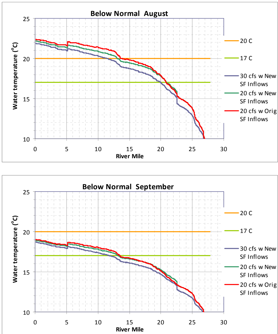
Figure 6b. Rubicon River below Normal Water Year Modeled Sensitivity Longitudinal Profiles—August (top) and September (bottom).
