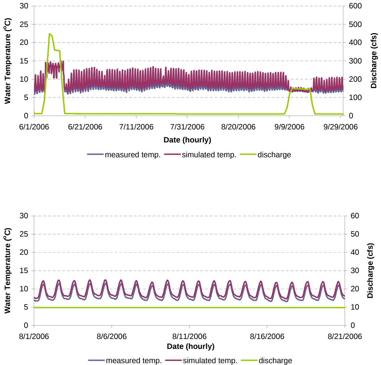
Figure F-1. Water Temperature Model Calibration Results for MF 46.6 in the French Meadows Reservoir to Middle Fork Interbay Reach of the Middle Fork American River for June 1 - September 30, 2006 (Top) and August 1 - August 21, 2006 (Bottom).
