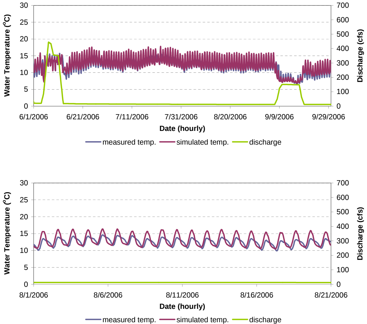
Figure F-3. Water Temperature Model Calibration Results for MF 44.6 in the French Meadows Reservoir to Middle Fork Interbay Reach of the Middle Fork American River for June 1 - September 30, 2006 (Top) and August 1 - August 21, 2006 (Bottom).
