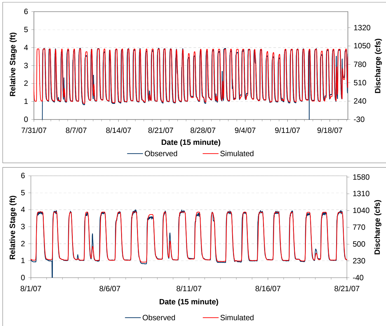
Figure AQ 4-18. RMA-2 Hydrodynamics Calibration Results for the Peaking Reach -- Otter Creek RM 14.5.
