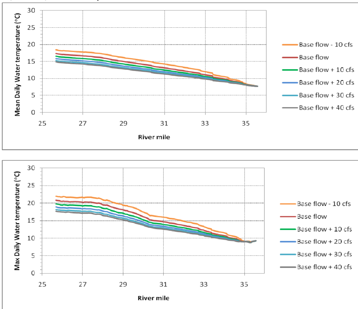
Figure H-10. Middle Fork American River from Middle Fork Interbay to Ralston Afterbay Longitudinal Profiles of Daily Mean (Top) and Maximum (Bottom) Water Temperature for the First Week of June, 2007 for Various Discharge Scenarios (-10 cfs, 0 cfs, +10 cfs, +20 cfs, +30 cfs, and +40 cfs).
