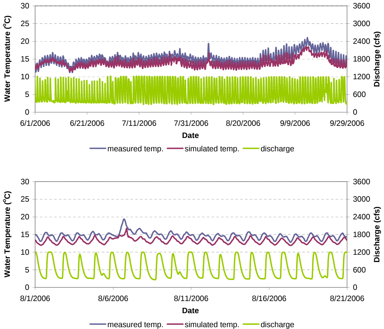
Figure F-45. Water Temperature Model Calibration Results for MF 0.1 in the Ralston Afterbay to Folsom Reservoir Reach of the Middle Fork American River for June 1 - September 30, 2006 (Top) and August 1 - August 21, 2006 (Bottom).
