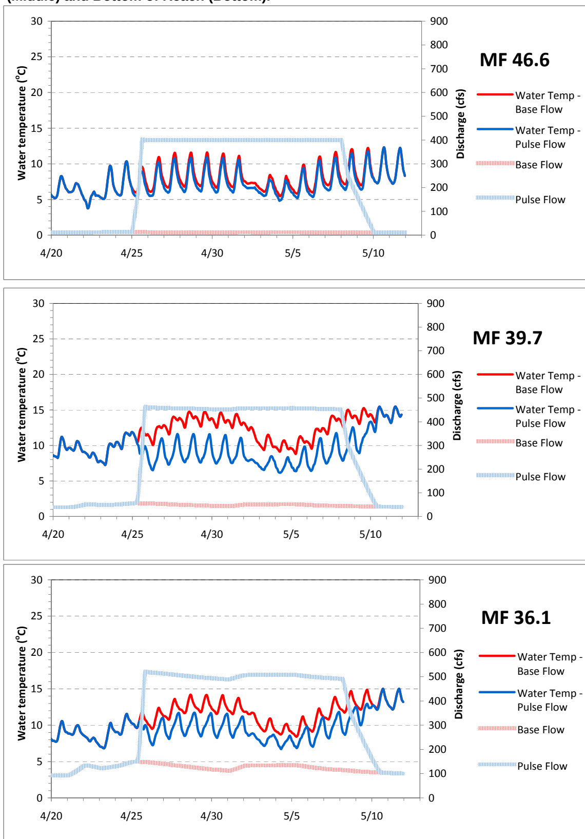
Figure H-8. Middle Fork American River from French Meadows Reservoir to Middle Fork Interbay Spring Pulse Flow Sensitivity Analysis for Top of Reach (Top), Middle of Reach (Middle) and Bottom of Reach (Bottom).
