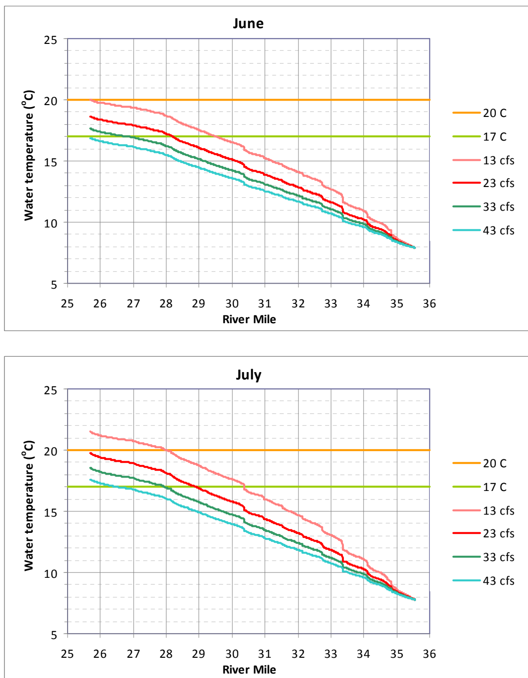
Figure 3a. Middle Fork American River below Middle Fork Interbay Modeled Sensitivity Longitudinal Profiles—June (top) and July (bottom)
