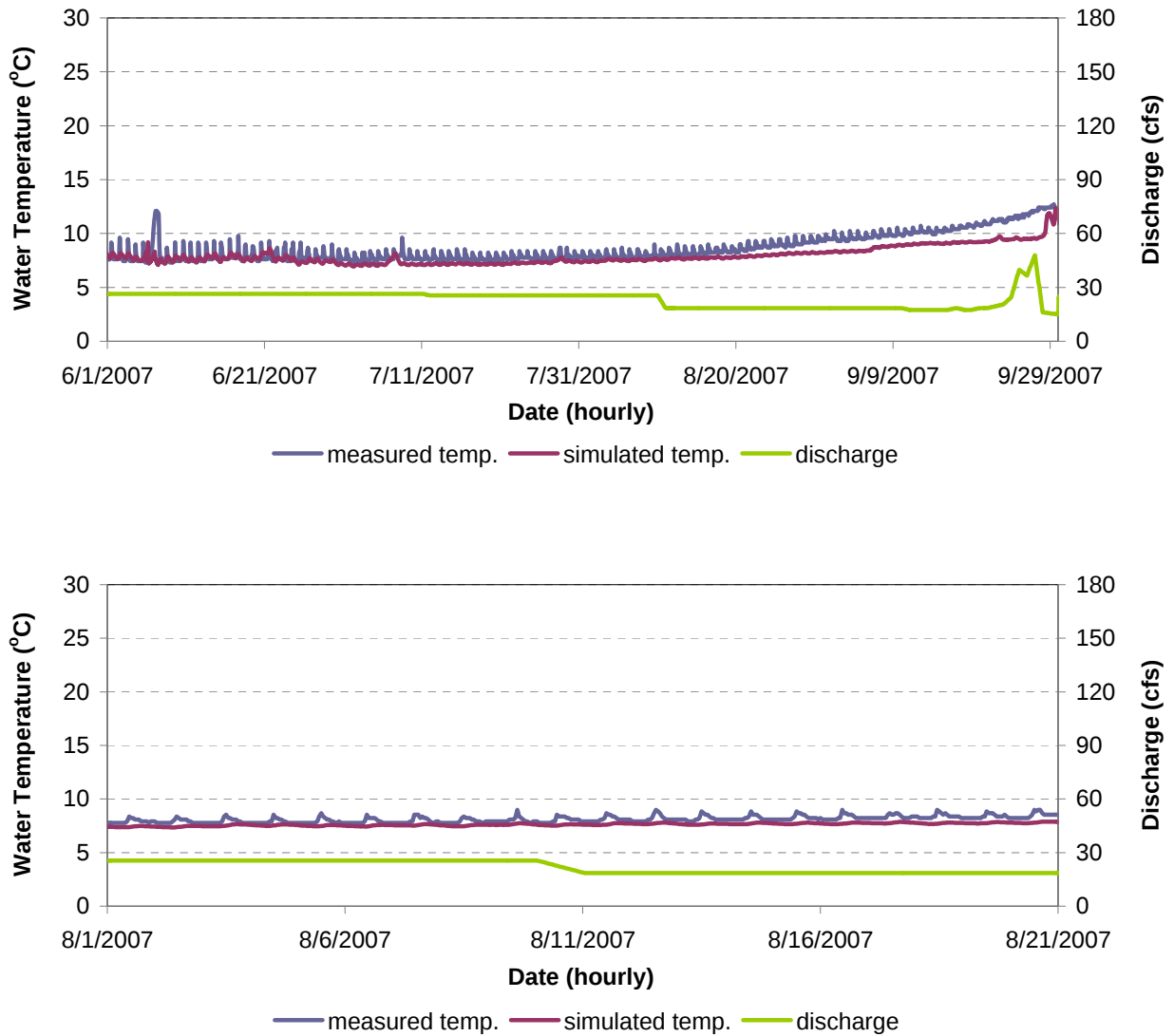
Figure F-10. Water Temperature Model Calibration Results for MF 35.5 in the Middle Fork Interbay to Ralston Afterbay Reach of the Middle Fork American River for June 1 - September 30, 2007 (Top) and August 1 - August 21, 2007 (Bottom).
