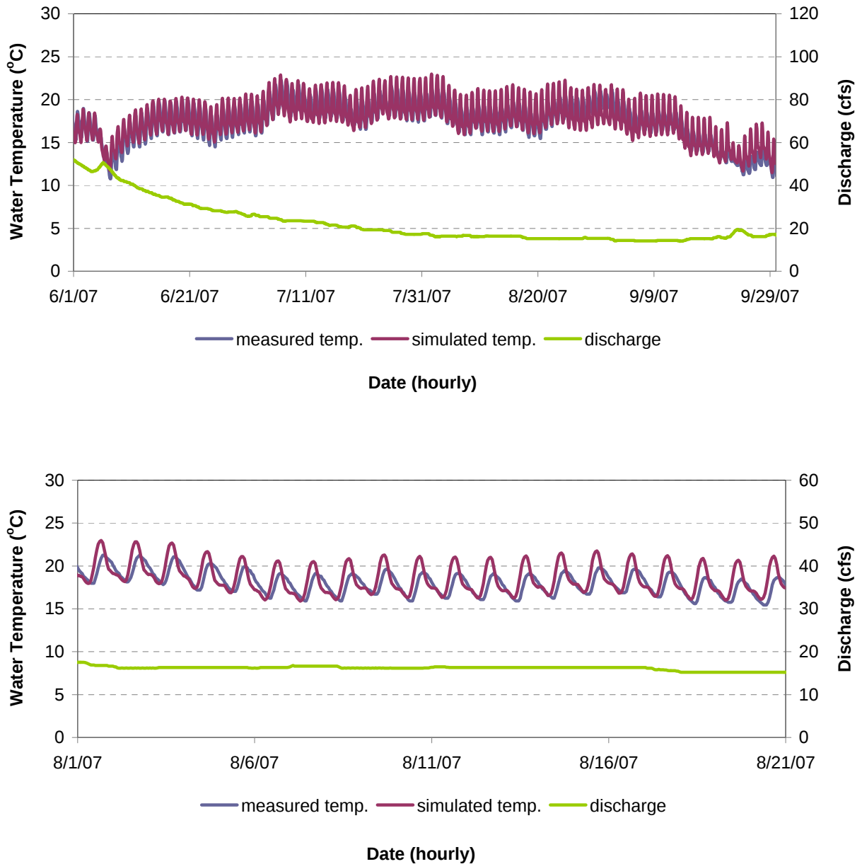
Figure F-8. Water Temperature Model Calibration Results for MF 36.1 in the French Meadows Reservoir to Middle Fork Interbay Reach of the Middle Fork American River for June 1 - September 30, 2007 (Top) and August 1 - August 21, 2007 (Bottom).
