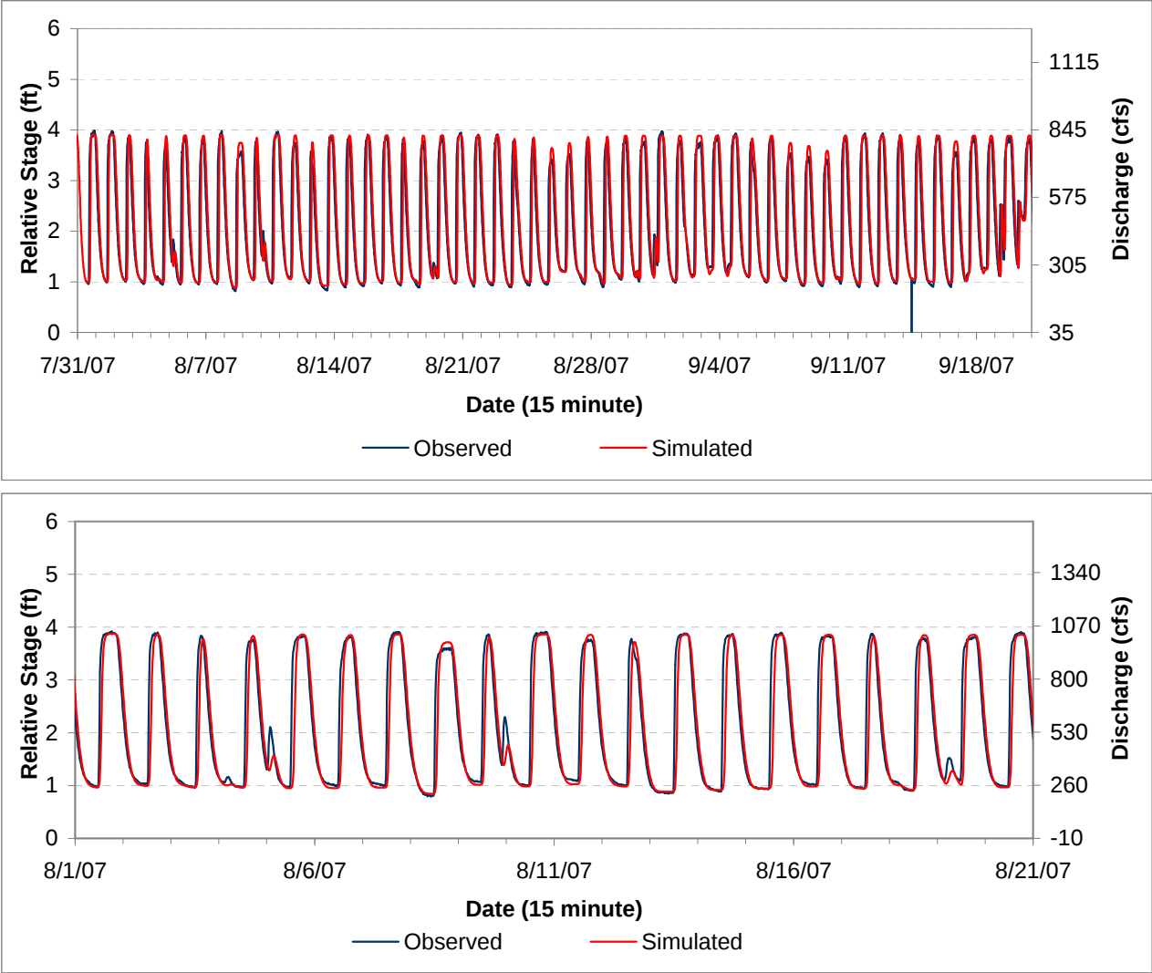
Figure AQ 4-20. RMA-2 Hydrodynamics Calibration Results for the Peaking Reach -- Below Mammoth Bar RM 1.4.
