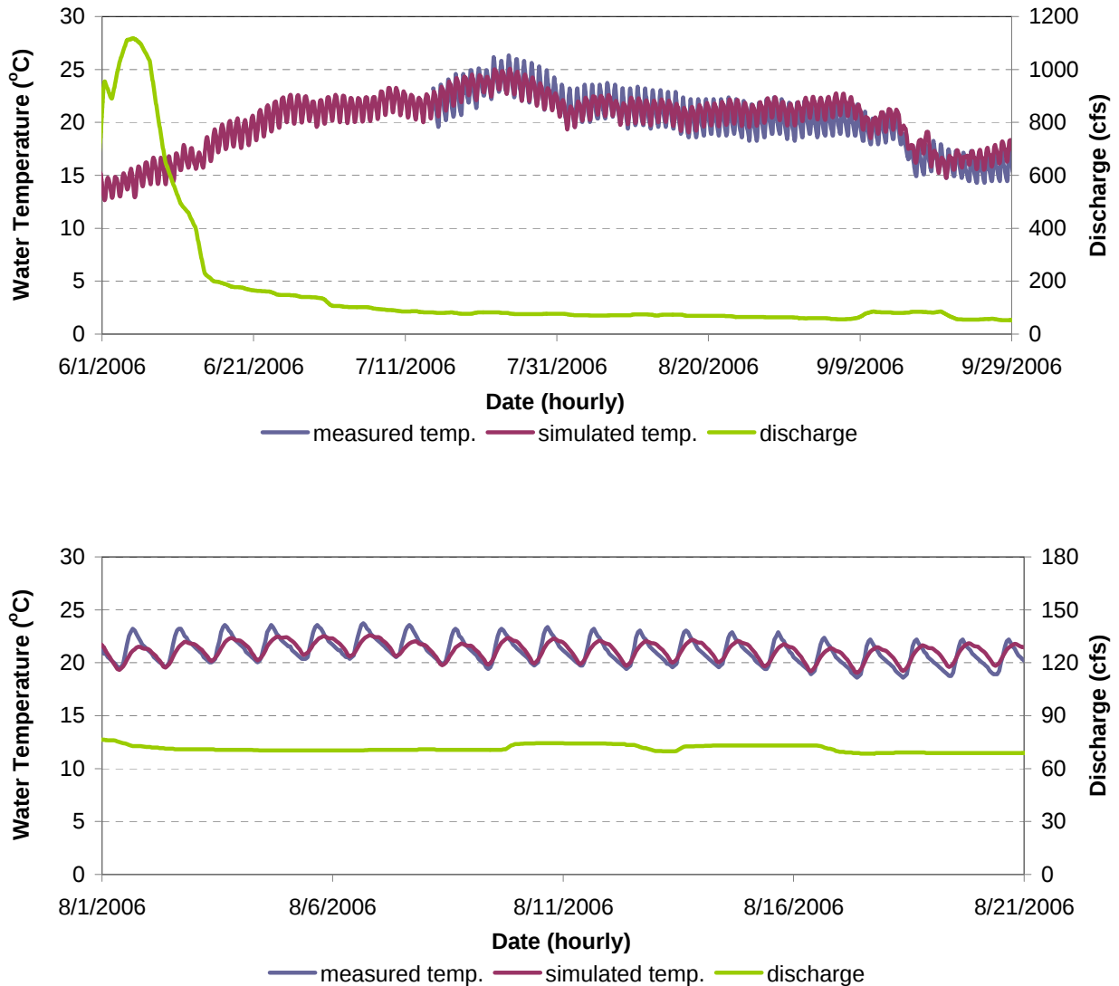
Figure F-27. Water Temperature Model Calibration Results for RR 3.7 in the Hell Hole Reservoir to Ralston Afterbay Reach of the Rubicon River for June 1 - September 30, 2006 (Top) and August 1 - August 21, 2006 Simulations (Bottom).
