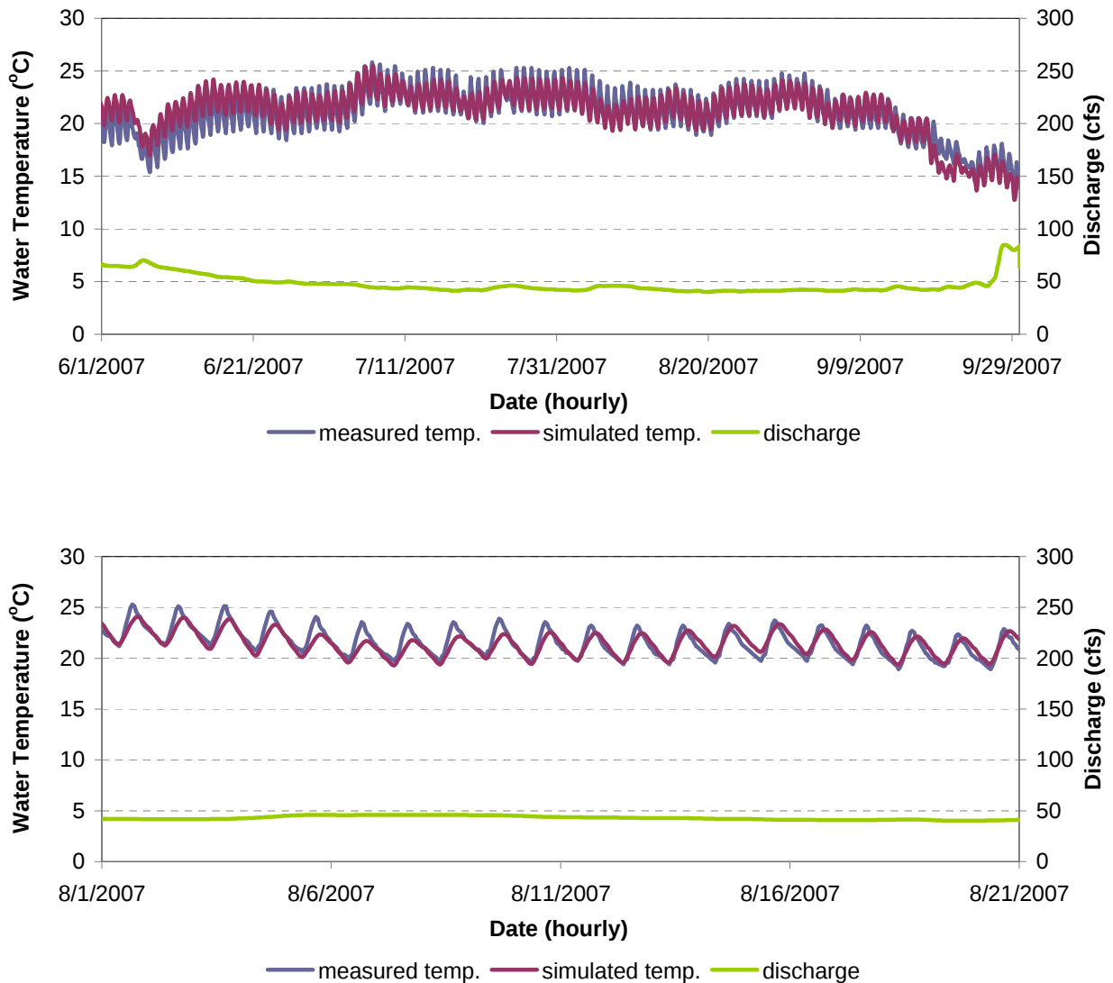
Figure F-28. Water Temperature Model Calibration Results for RR 3.7 in the Hell Hole Reservoir to Ralston Aferbay Reach of the Rubicon River for June 1 - September 30, 2007 (Top) and August 1 - August 21, 2007 (Bottom).
