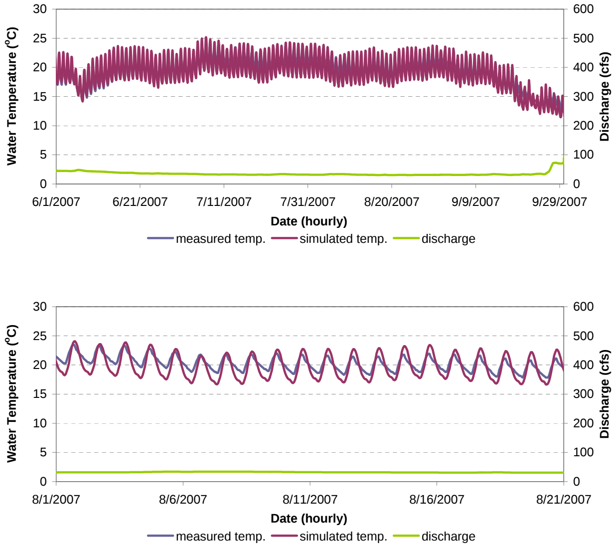
Figure F-24. Water Temperature Model Calibration Results for RR 14.3 in the Hell Hole Reservoir to Ralston Afterbay Reach of the Rubicon River for June 1 - September 30, 2007 (Top) and August 1 - August 21, 2007 (Bottom).
