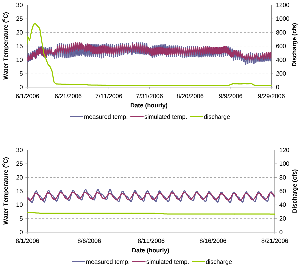
Figure F-17. Water Temperature Model Calibration Results for RR 25.3 in the Hell Hole Reservoir to Ralston Afterbay Reach of the Rubicon River for June 1 - September 30, 2006 (Top) and August 1 - August 21, 2006 (Bottom).
