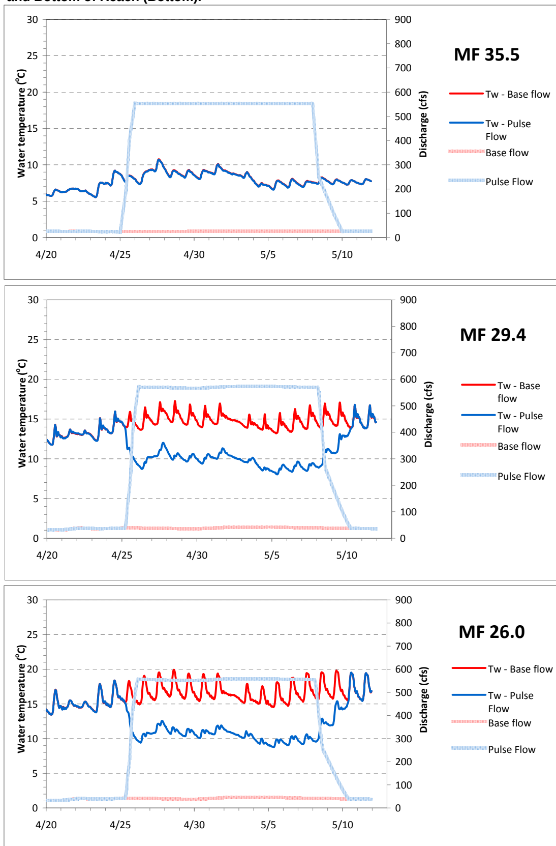
Figure H-16. Middle Fork American River from Middle Fork Interbay to Ralston Afterbay Spring Pulse Flow Sensitivity Analysis for Top of Reach (Top), Middle of Reach (Middle) and Bottom of Reach (Bottom).
