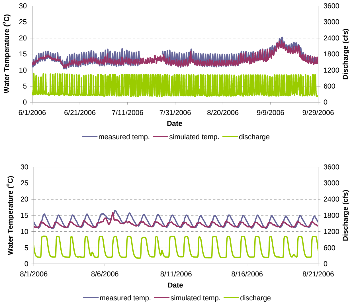
Figure F-41. Water Temperature Model Calibration Results for MF 11.0 in the Ralston Afterbay to Folsom Reservoir Reach of the Middle Fork American River for June 1 - September 30, 2006 (Top) and August 1 - August 21, 2006 (Bottom).
