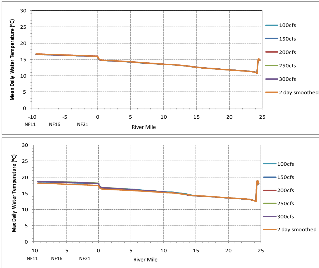
Figure H-31. Middle Fork American River Peaking Reach Longitudinal Profiles of Daily Mean (Top) and Maximum (Bottom) Water Temperature for the First Week of August, 2007 for Various Discharge Scenarios (100 cfs, 150 cfs, 200 cfs, 250 cfs and 300 cfs Minimum Discharge and 2-Day Average Discharge).
