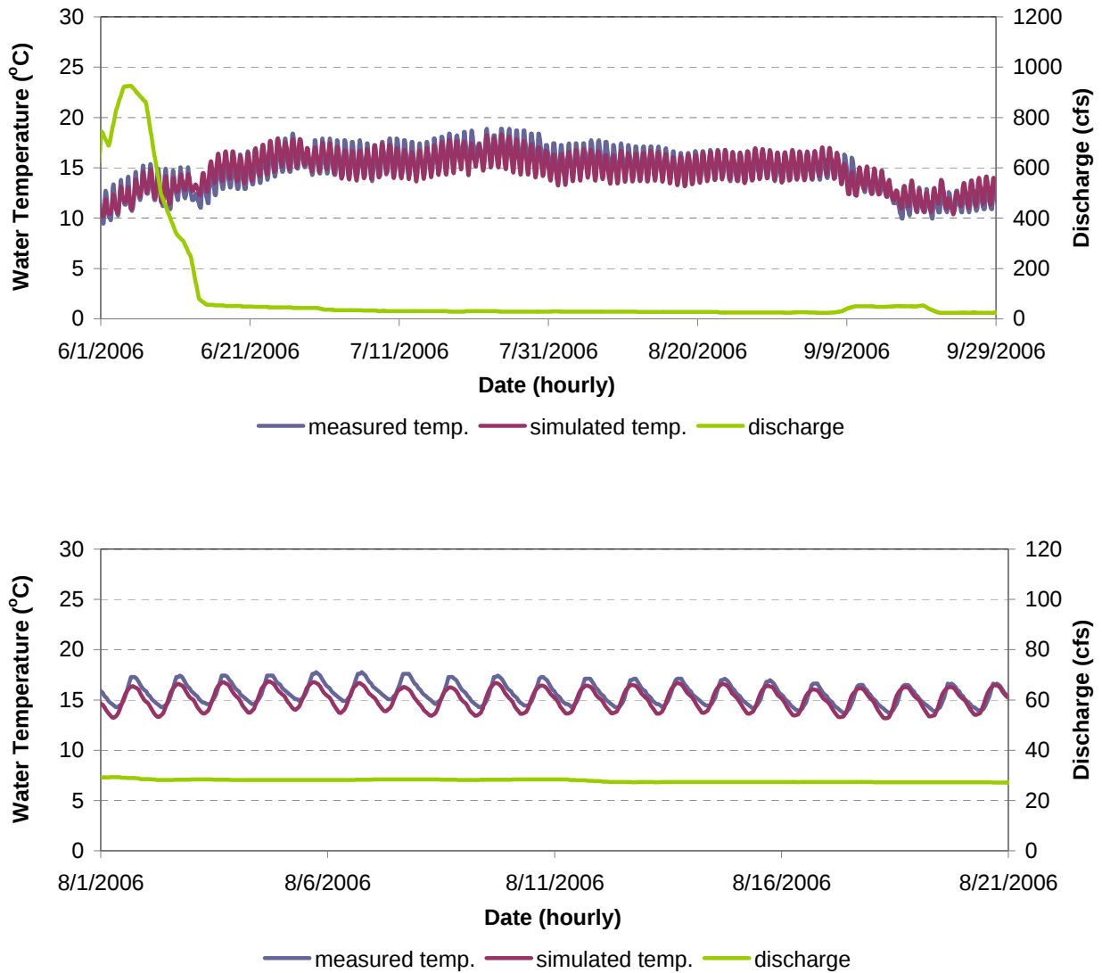
Figure F-19. Water Temperature Model Calibration Results for RR 22.7 in the Hell Hole Reservoir to Ralston Afterbay Reach of the Rubicon River for June 1 - September 30, 2006 (Top) and August 1 - August 21, 2006 (Bottom).
