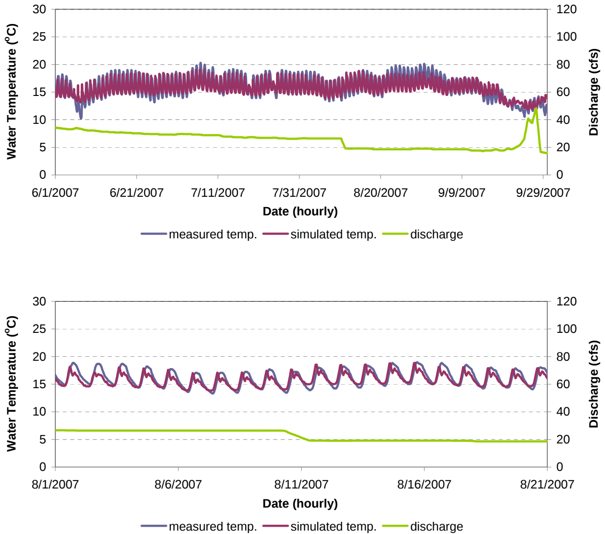
Figure F-12. Water Temperature Model Calibration Results for MF 29.4 in the Middle Fork Interbay to Ralston Afterbay Reach of the Middle Fork American River for June 1 - September 30, 2007 (Top) and August 1 - August 21, 2007 (Bottom).
