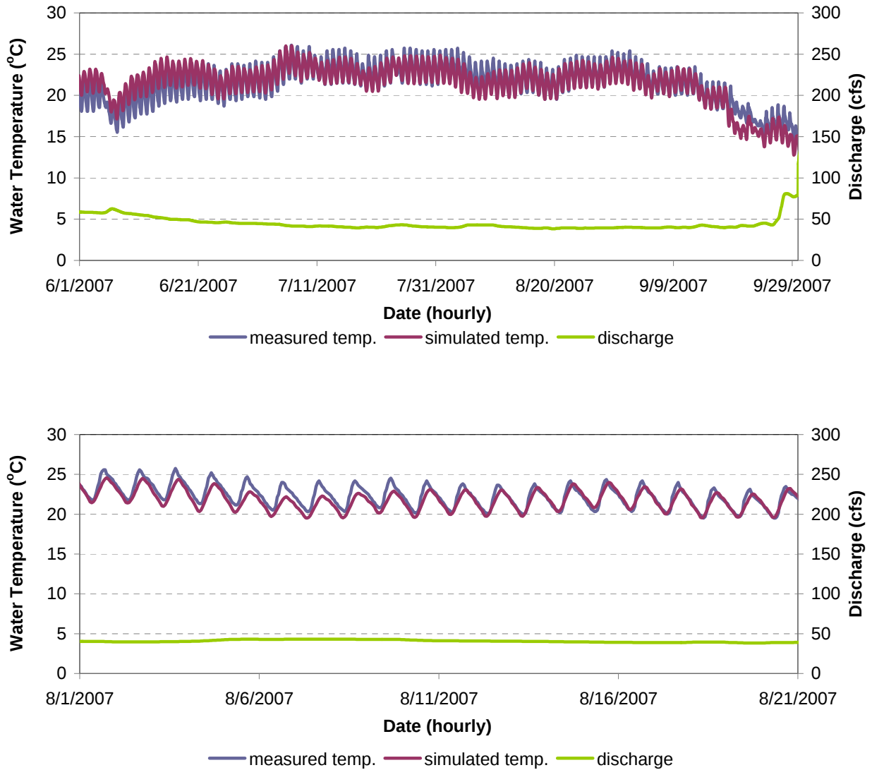
Figure F-26. Water Temperature Model Calibration Results for RR 5.3 in the Hell Hole Reservoir to Ralston Afterbay Reach of the Rubicon River for June 1 - September 30, 2007 (Top) and August 1 - August 21, 2007 (Bottom).
